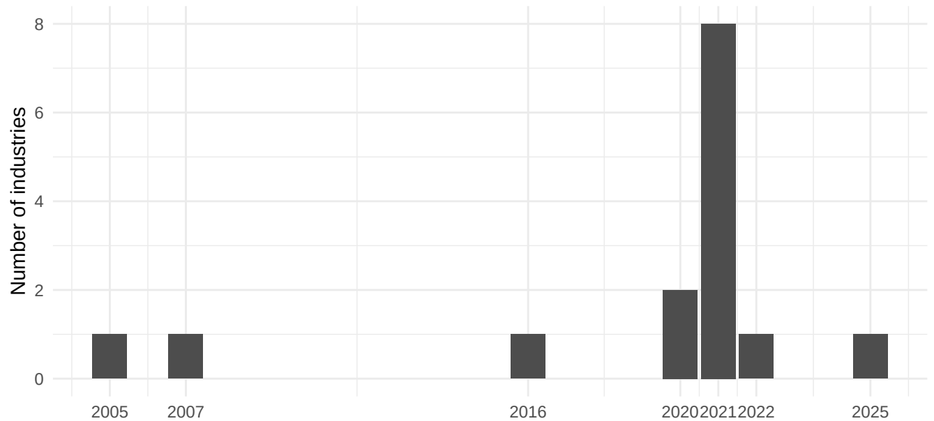
Estimated structural-break years (Zivot-Andrews)
