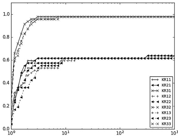
Fig. 1. Fraction of problems solved vs error factor for LHS design of size 1.
