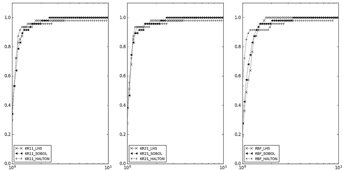
Fig. 5. Fraction of problems solved vs error factor for different sampling designs starting with size of 'size 2'.
