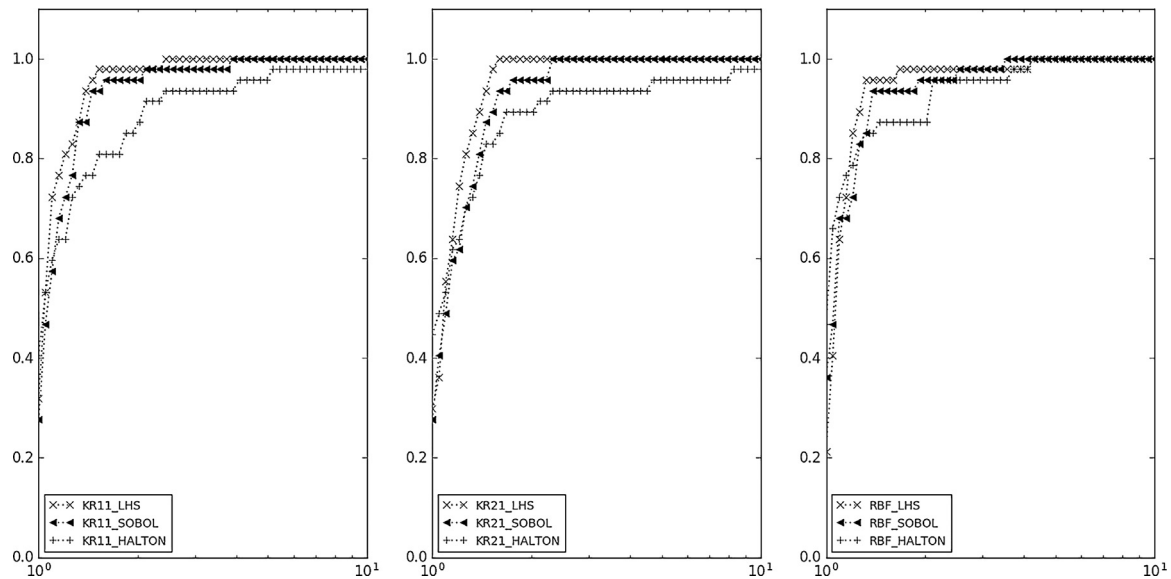
Fig. 4. Fraction of problems solved vs error factor for different sampling designs starting with size of 'size 1'.
