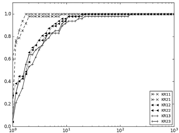
Fig. 2. Fraction of problems solved vs error factor for LHS design of size 1.
