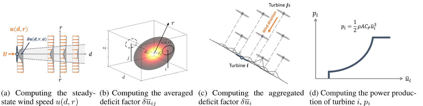
Fig. 1. Engineering-based wake modelling steps.
