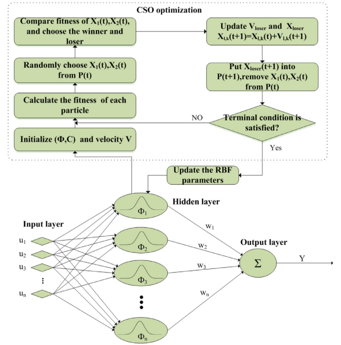
Fig. 2. Procedure of CSO optimized RBF network.
