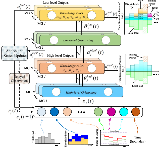
Fig. 2. The overall framework design of HRL.
