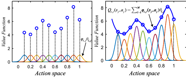
Fig. 3. Schematic diagram of RBF approximating one-dimensional Q function.
