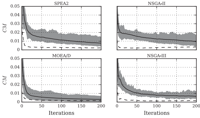
Fig. 8. Dynamic plots of CM versus iterations for SPEA2, NSGA-II, MOEA/D and NSGA-III for 50 random seed trial runs. The range of CM is indicated by the shaded region, the mean by a solid line, and the standard deviation by a dashes line.
