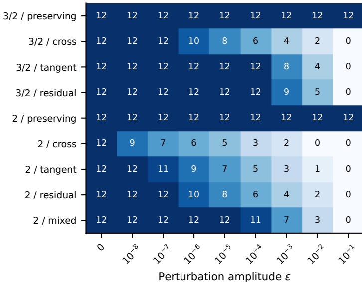
(a) Eligible radii / 12
