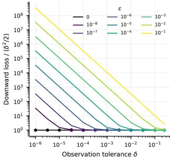
(b) Quadratic task + cross leakage
