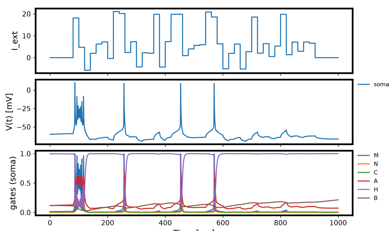
Raw training trajectories.
