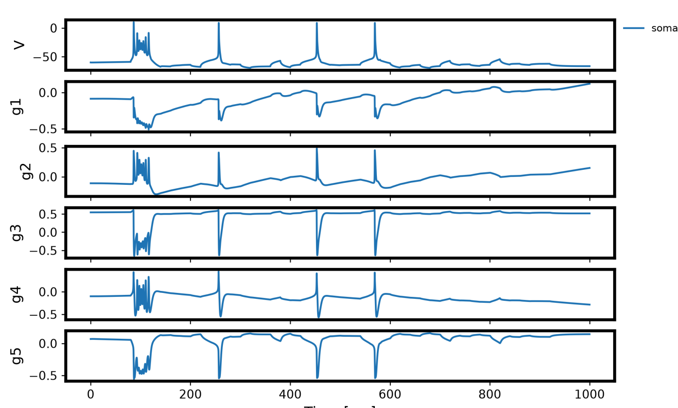
Latent trajectories used to fit the SINDy library.
