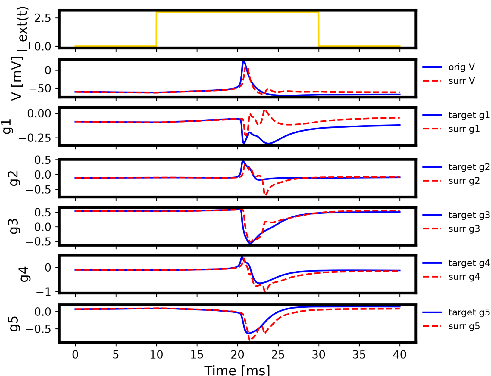
20 ms, 3 \mu A/cm 2 step: V and the 5 AE latents .
