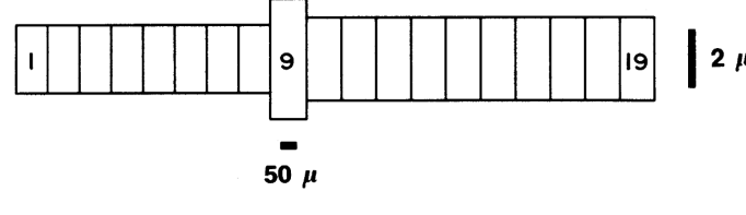
Pyramidal neuron [1]
