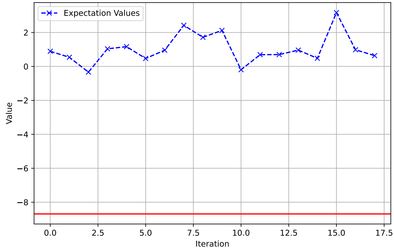
Ground state energy
