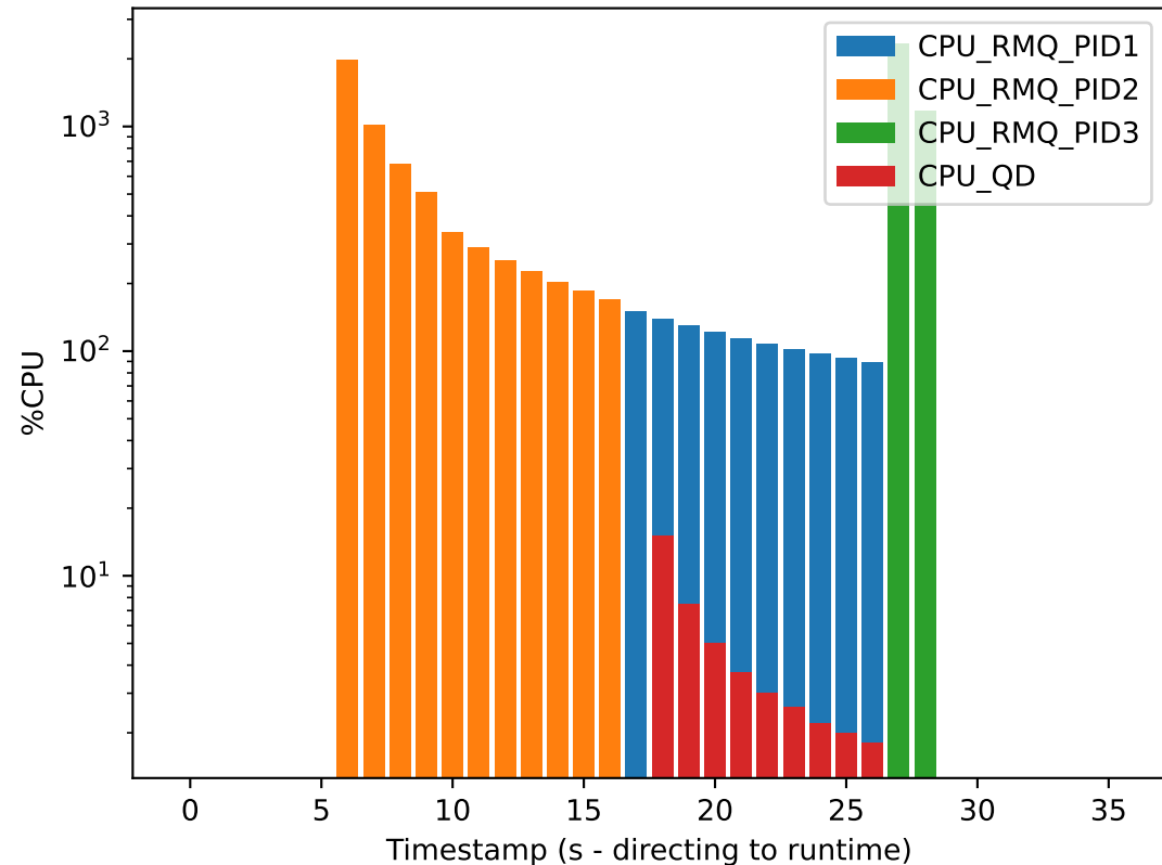
CPU Percentage of RabbitMQ and Qdaemon
