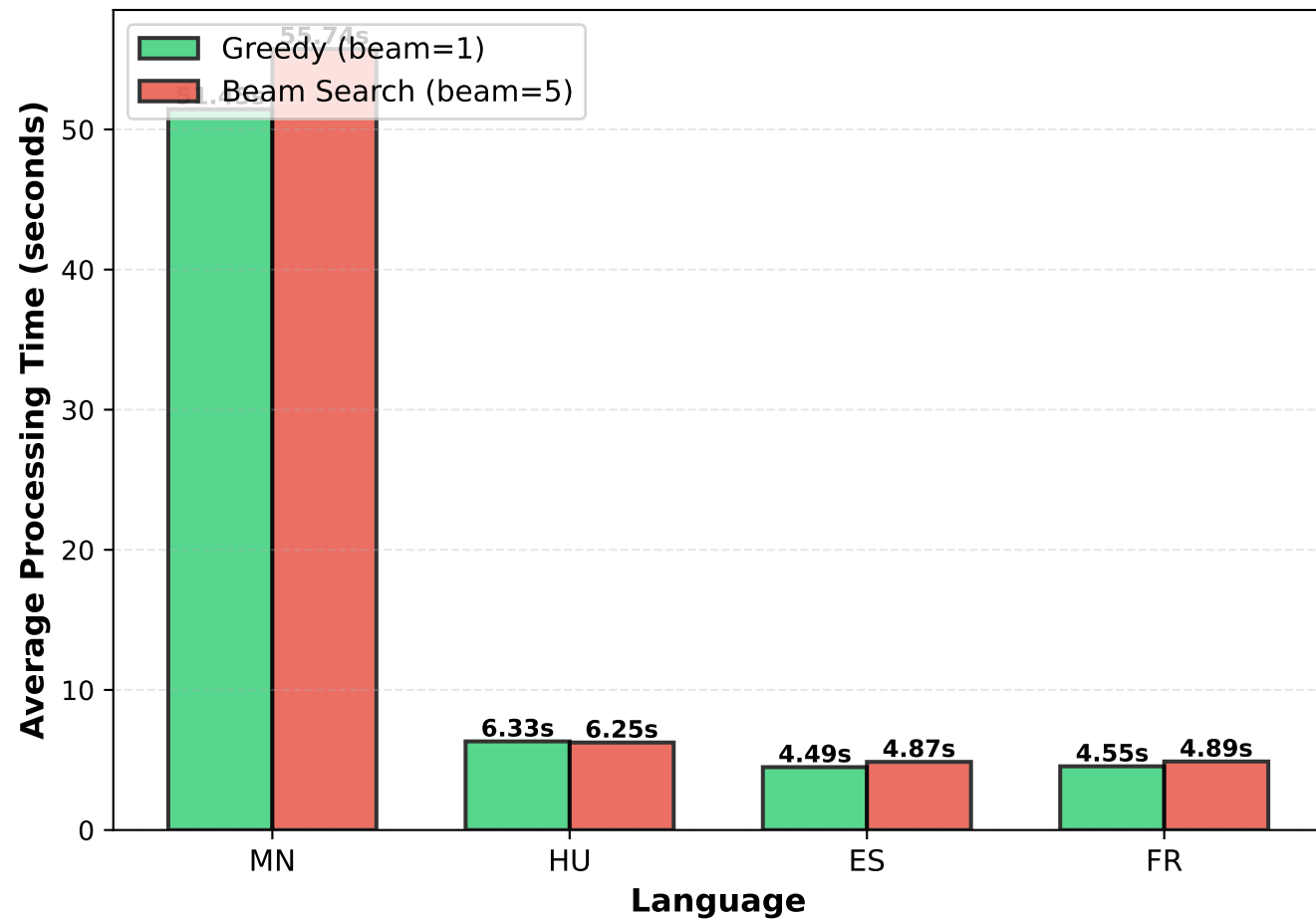
Greedy vs Beam Search Decoding (5 files per language, Whisper-small, CPU)
