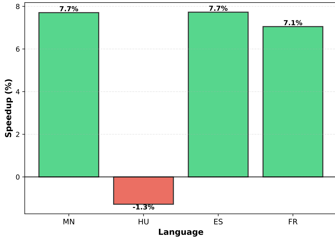
Greedy Speedup vs Beam Search (Positive = Greedy is Faster)
