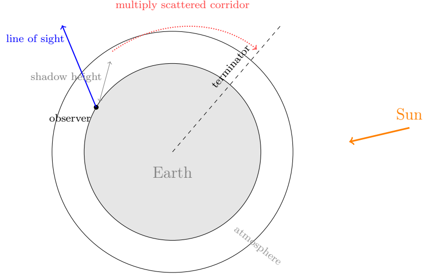
Figure 1: The deep-twilight geometry: beyond \text{SZA} \sim 96^\circ the observer’s entire line of sight lies inside the Earth’s shadow; the observable radiance is carried by photons scattered at high altitude on the sunlit side of the terminator, transported laterally, and scattered again into the line of sight (backward chains must discover this corridor in reverse). Every variance-reduction component of Section 3 exists to sample this corridor efficiently without bias.
