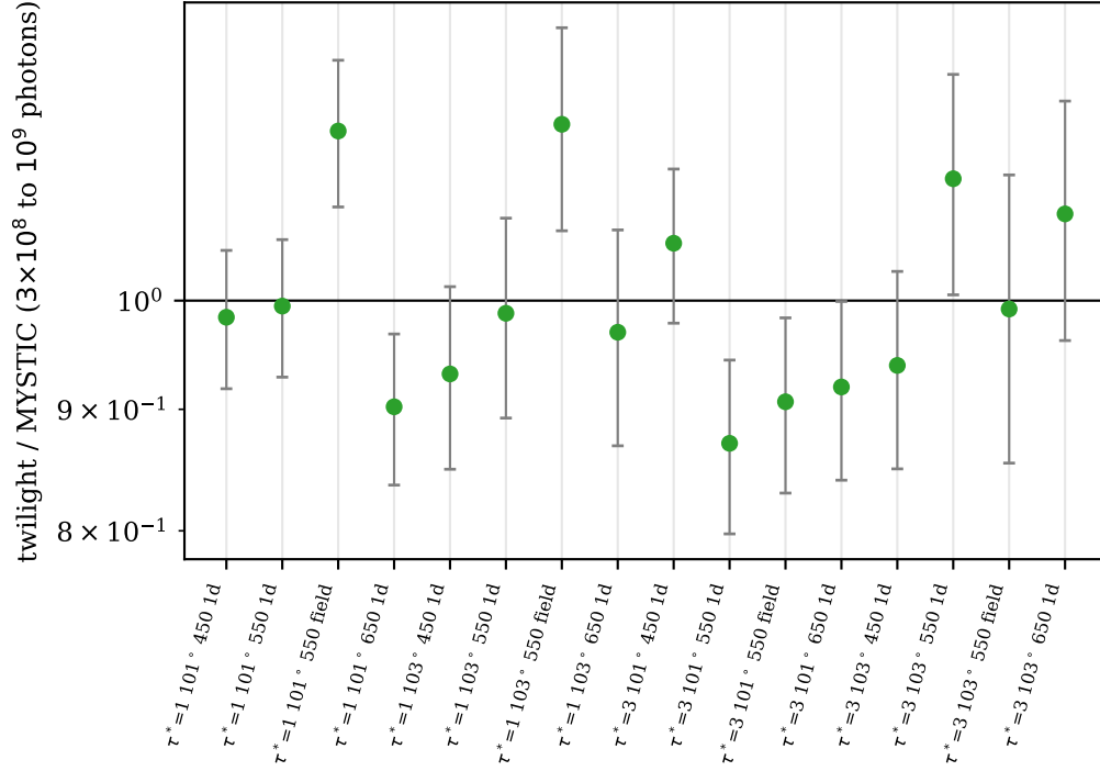
Figure 6: Every cell of the deep-regime referee table, shown as the model-to-MYSTIC ratio with combined error bars (model seed SE and referee SE propagated in quadrature); referee budgets are 3 \times 10^8 to 10^9 photons. All sixteen cells, the one-dimensional and the three-dimensional field paths alike, are gated and statistically consistent (green; ratios 0.87 to 1.19). The field cells referee the voxel path on the equivalent horizontally uniform field of the same deck and share the one-dimensional rows' reference values; the two at SZA 103^\circ , low-power at earlier seed budgets, close at 1024 and 512 seeds with the field estimator unchanged.
