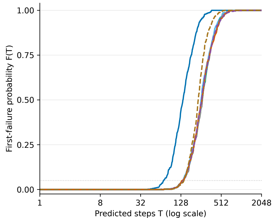
Model seed 0 (26/26 arms)
