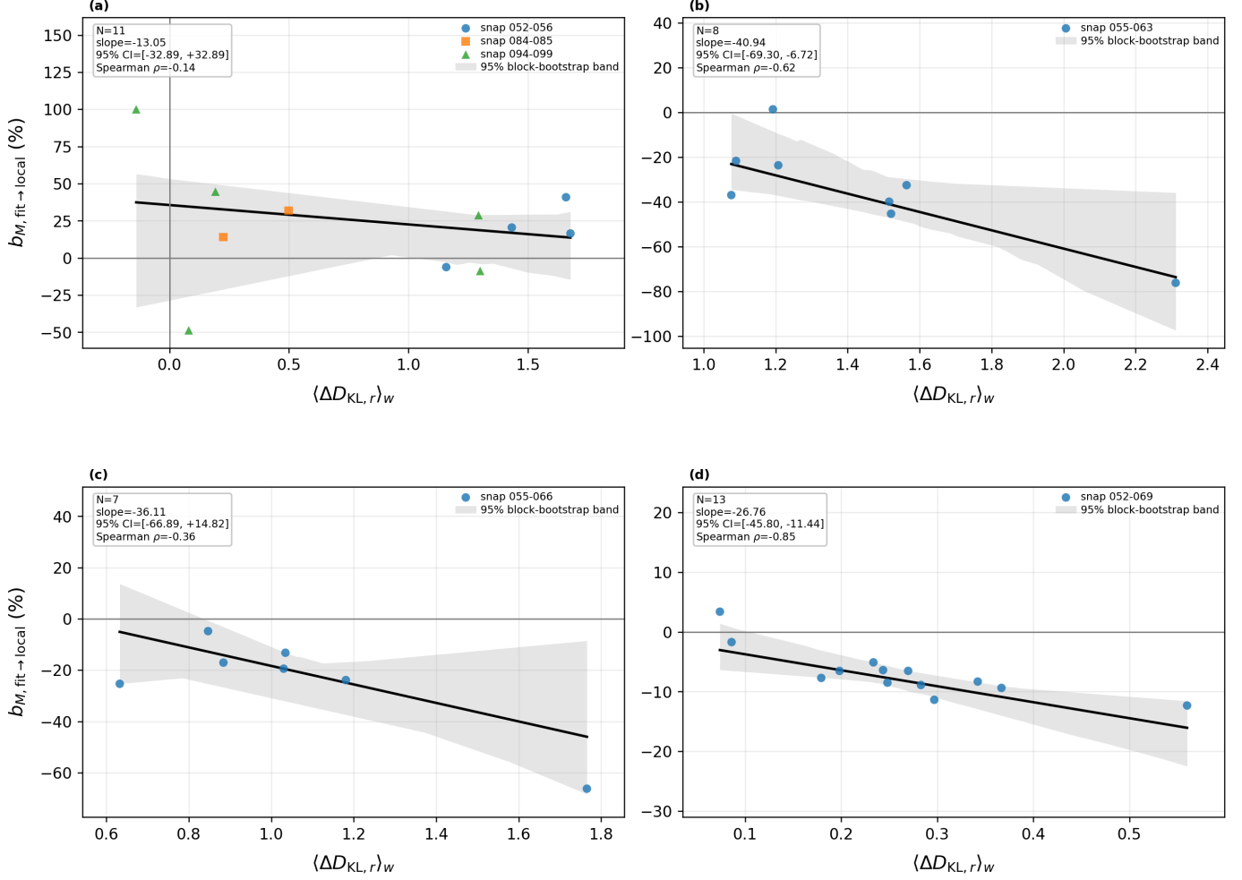
Figure 5. Fitted-to-reference enclosed-mass bias, b_{M, \text{fit} \rightarrow \text{local}} , versus the matched-star-count-weighted fitted-minus-BFE clustering difference, \langle \Delta D_{KL,r} \rangle_w , for the BFE-valid 80–100 kpc snapshot intervals. Panels (a)–(d) show the 1:2, 1:5, 1:10, and 1:100 mergers, respectively. Each point represents one snapshot, and different marker shapes distinguish disconnected contiguous BFE-valid intervals. Black lines show Theil–Sen robust linear fits, while the gray regions show the 95% moving-block-bootstrap confidence bands, which account approximately for temporal correlation between neighboring snapshots. The annotation boxes give the number of plotted snapshots, the fitted slope and its bootstrap interval, and the Spearman rank coefficient. The fits quantify the empirical association between orbit-integrated action-structure disagreement and recovery of the local spherical reference over the analyzed intervals.
