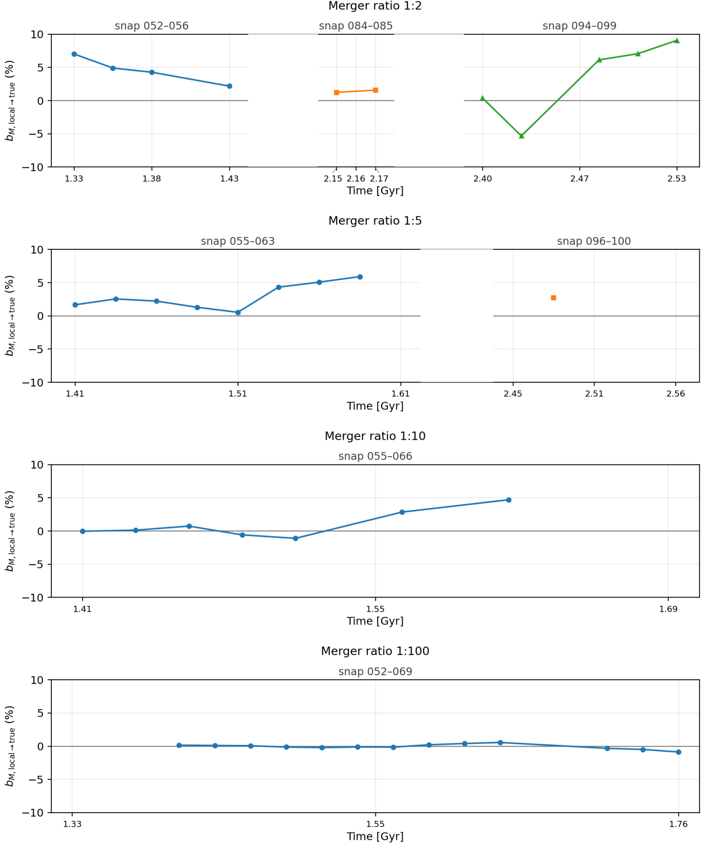
Figure 7. Reference-to-global contribution to the enclosed-mass bias, b_{M, \text{local} \rightarrow \text{true}} , evaluated using the selected outer-range cohorts during the BFE-valid snapshot intervals. From top to bottom, the rows show the 1:2, 1:5, 1:10, and 1:100 mergers. At each radial grid point, the locally sampled spherical-equivalent mass is inferred from the BFE radial force over the angular region occupied by the selected cohorts and is compared with the globally spherically averaged BFE enclosed mass. Disconnected segments and different marker styles identify separate contiguous BFE-valid intervals. The mismatch remains mostly below 10% even for the 1:2 merger and is generally only a few percent for the weaker mergers. Thus, the force-based local spherical reference remains close to the global spherical average, and most of the larger total mass bias lies between the KLD-fitted and local reference profiles.
