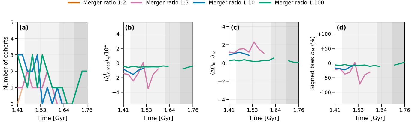
Figure 8. Comparison of the KLD-fitted spherical NFW model with the frozen-snapshot BFE field for merger mass ratios 1:2, 1:5, 1:10, and 1:100 in the 80 \leq r/\text{kpc} \leq 100 radial range. Only BFE-valid snapshot intervals within 1.41 \leq t/\text{Gyr} \leq 1.76 contribute to the comparison. (a) Number of selected coherent cohorts. The color identifies the merger ratio. The saturation of each curve segment encodes the average stellar membership of the selected cohorts, which typically ranges from 870 to 950; more saturated segments correspond to larger average membership. (b) Matched-star-count-weighted signed median displacement, \langle \Delta \tilde{J}_{r,\text{med}} \rangle_w , scaled by 10^4 as indicated on the axis. (c) Matched-star-count-weighted signed clustering difference, \langle \Delta D_{\text{KL},r} \rangle_w . (d) Signed enclosed-mass bias, b_M , of the fitted spherical model relative to the globally spherically averaged BFE mass profile. The action diagnostics are defined in Equations 75 and 76. The displayed time range is chosen to maximize overlapping BFE-valid coverage across the merger cases and therefore does not encompass the principal BFE-valid interval of every individual simulation. The 1:2 merger is consequently underrepresented in this comparison. White background indicates times at which all four merger cases lie within BFE-valid intervals; progressively darker gray indicates that fewer cases provide a valid BFE comparison. Missing action- or mass-diagnostic segments occur when the BFE comparison is unavailable or when no selected cohort contributes a finite measurement at that time.
