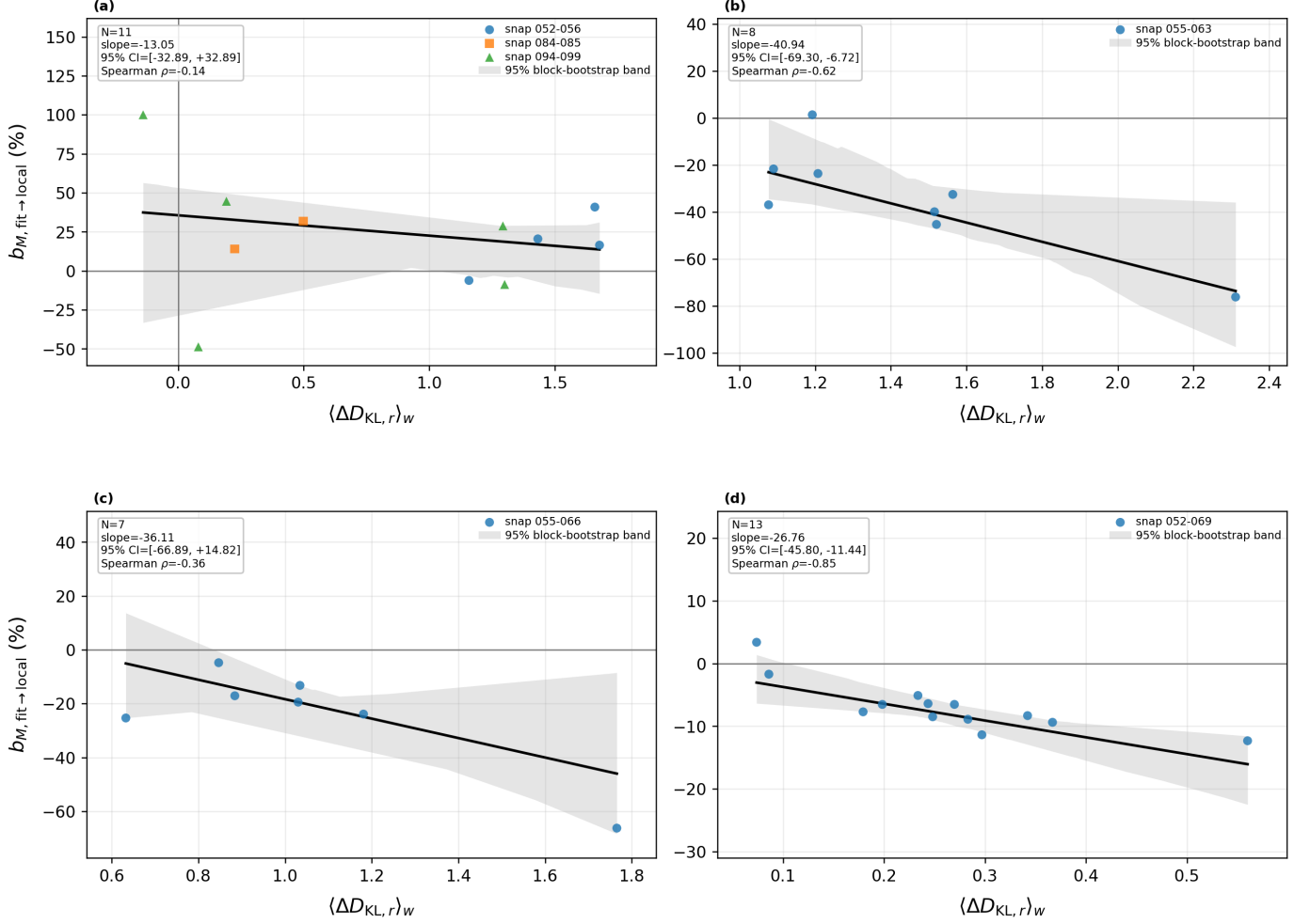
Figure 5. Fitted-to-reference enclosed-mass bias, b_{M,\text{fit} \rightarrow \text{local}} , versus the matched-star-count-weighted fitted-minus-BFE clustering difference, \langle \Delta D_{\text{KL},r} \rangle_w , for the BFE-valid 80–100 kpc snapshot intervals. Panels (a)–(d) show the 1:2, 1:5, 1:10, and 1:100 mergers, respectively. Each point represents one snapshot, and different marker shapes distinguish disconnected contiguous BFE-valid intervals. Black lines show Theil–Sen robust linear fits, while the gray regions show the 95% moving-block-bootstrap confidence bands, which account approximately for temporal correlation between neighboring snapshots. The annotation boxes give the number of plotted snapshots, the fitted slope and its bootstrap interval, and the Spearman rank coefficient. The fits quantify the empirical association between orbit-integrated action-structure disagreement and recovery of the local spherical reference over the analyzed intervals.
