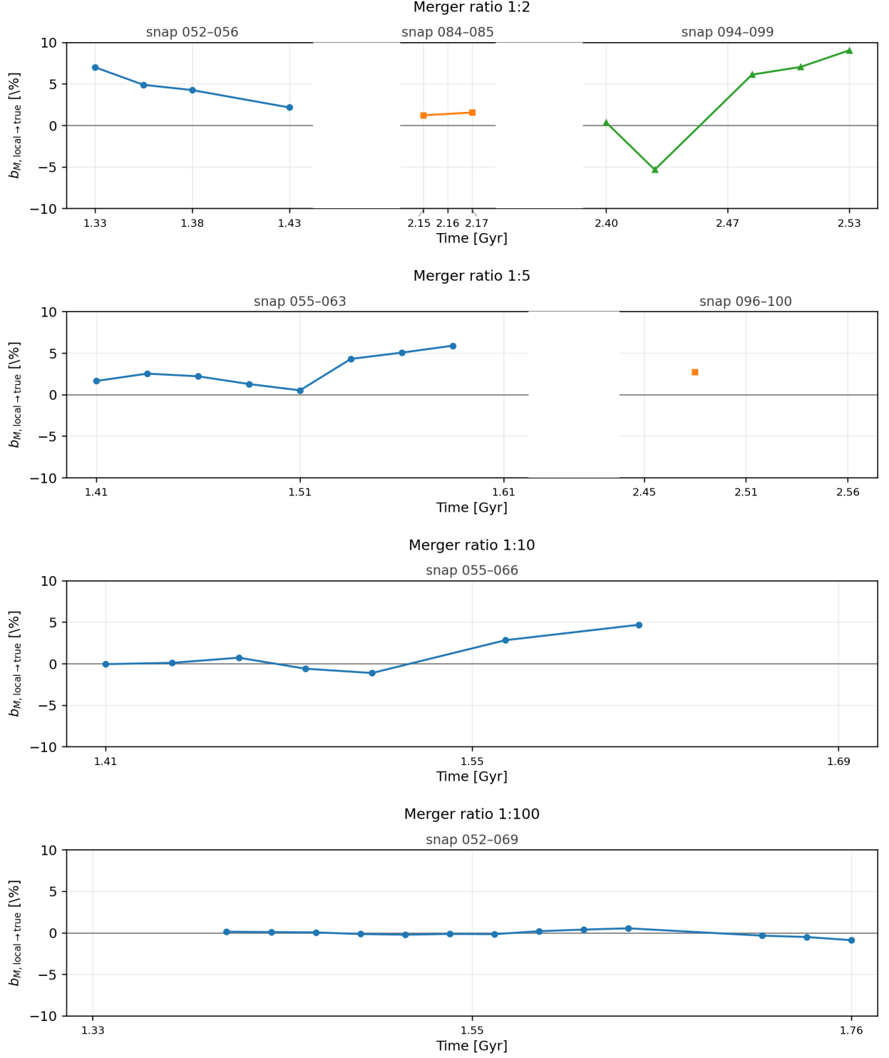
Figure 8. Local-to-true contribution to the enclosed-mass bias, b_{M, \text{local} \rightarrow \text{true}} , evaluated over the outer-range cohorts in the BFE-valid snapshot intervals. Each curve compares the spherical-equivalent mass inferred from the local BFE potential in the space sampled by the selected cohorts. The mismatch remains mostly below 10% even for the 1:2 merger and is generally only a few percent for the weaker mergers. Thus, merger-induced non-sphericity contributes to the total mass bias but is typically subdominant to the discrepancy between the KLD-fitted potential and the locally sampled BFE field.
