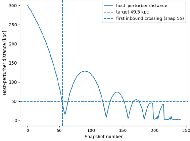
Figure 2. Plot for host-perturber distance for the simulation of tidal streams in the Milky Way under an LMC-like merger. Snapshot 55 ( t = 1.406 Gyr) is identified as the distance-matched present-day reference snapshot.
