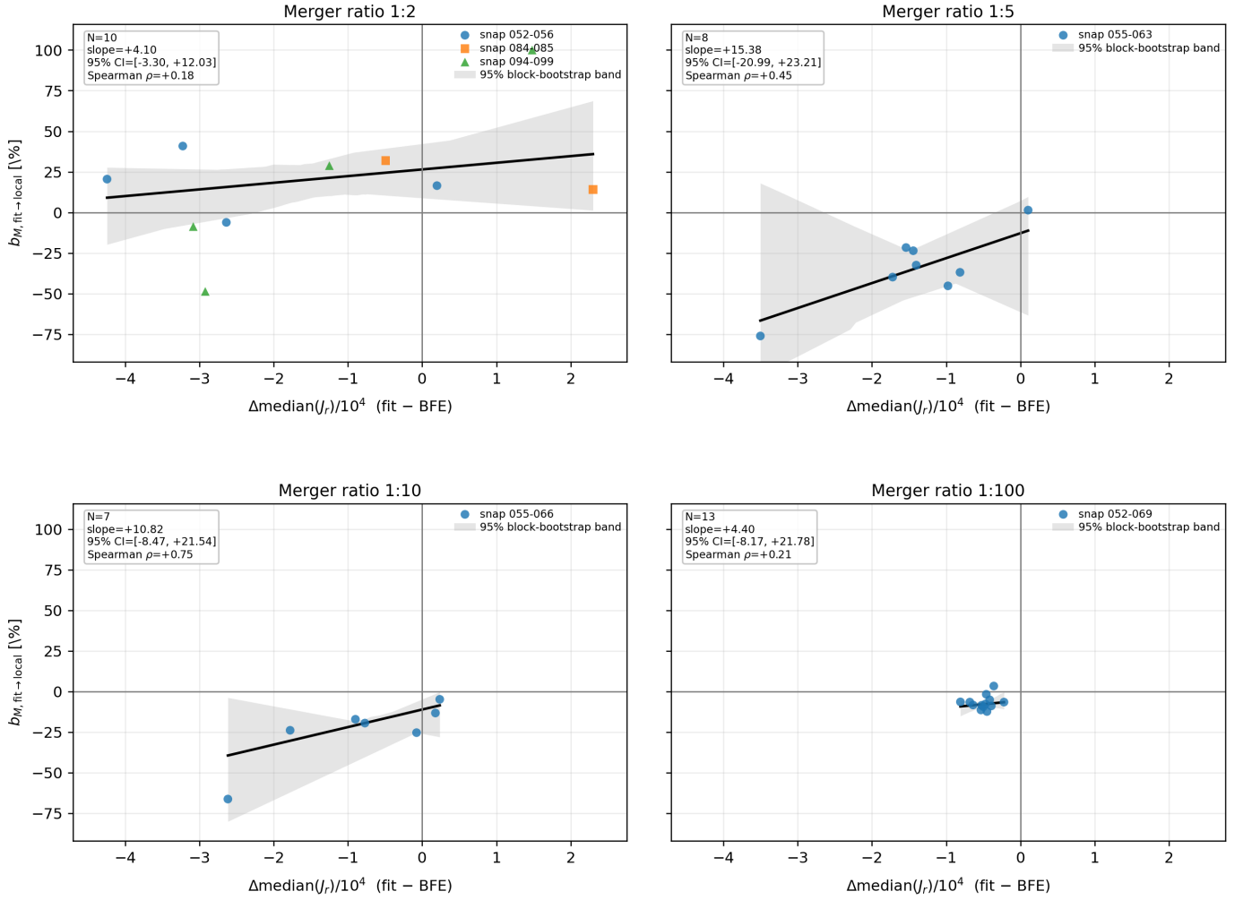
Figure 7. Fit-to-local enclosed-mass bias, b_{M, \text{fit} \rightarrow \text{local}} , versus signed fitted-minus-BFE action-cloud displacement \Delta \text{median}(J_r) = \text{median}(J_{r, \text{fit}}) - \text{median}(J_{r, \text{BFE}}) for the 1:2, 1:5, 1:10, and 1:100 mergers in the BFE-valid 80-100 kpc snapshot intervals. The 1:2 case exhibits only shallow scalar trends.
