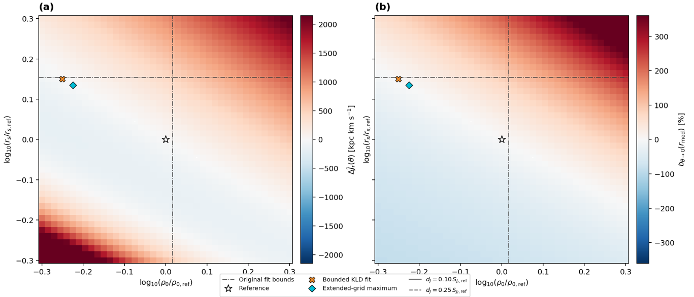
Figure 10. Median-action degeneracy for the same 1:10 cohort, snapshot, and radial range as Figure 9. (a) Signed difference between the median radial action in each trial potential and that in the reference potential, \Delta \text{median } J_r(\theta) . The contour marks |\Delta \text{median } J_r| = 0.10 S_{J_r, \text{ref}} , where S_{J_r, \text{ref}} is the MAD width of the reference radial-action cloud. It therefore identifies the boundary of the region whose median action is close to the reference median under the adopted tolerance. (b) Signed enclosed-mass difference b_{\theta \rightarrow 0}(r_{\text{med}}) over the same parameter grid. The extended reference-median-equivalent region demonstrates that recovery of the reference median action does not uniquely recover the reference NFW parameters. Gray pixels indicate trial potentials for which the finite-action requirement is not satisfied.
