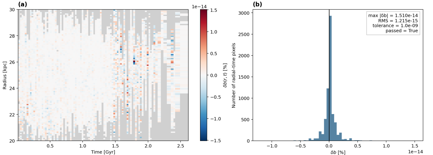
Figure 6. Numerical closure test for the mass-bias decomposition in Figure 5. (a) Closure residual \delta b(r, t) over the valid radius–time pixels. The color scale is of order 10^{-14} percentage points. (b) Distribution of the valid closure residuals. The maximum absolute residual is 1.510 \times 10^{-14} percentage points and the RMS residual is 1.215 \times 10^{-15} percentage points, both far below the adopted 10^{-9} tolerance. Gray regions in panel (a) indicate pixels for which the component biases are unavailable.
