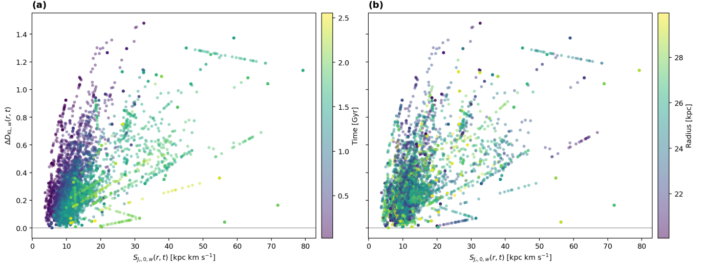
Figure 7. Relation between the weighted reference radial-action spread, S_{Jr,0,w} , and the weighted KLD excess, \Delta D_{\text{KL},w} , for the 1:10 merger in the 20 \leq r/\text{kpc} \leq 30 radial range. Each point represents one valid radius-snapshot measurement. The points are colored by snapshot time in panel (a) and by radius in panel (b). Positive \Delta D_{\text{KL},w} indicates that the KLD fit produces a more strongly clustered action cloud than the reference potential. The distribution broadens toward larger KLD excess as the reference action cloud becomes more extended, although the relation contains substantial intrinsic scatter.
