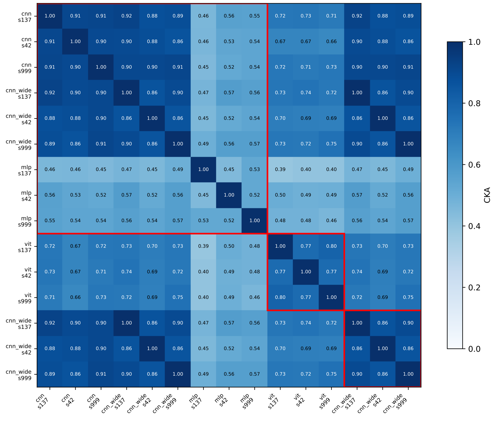
CKA Matrix: Within- and Cross-Architecture (Red boxes = same architecture)
