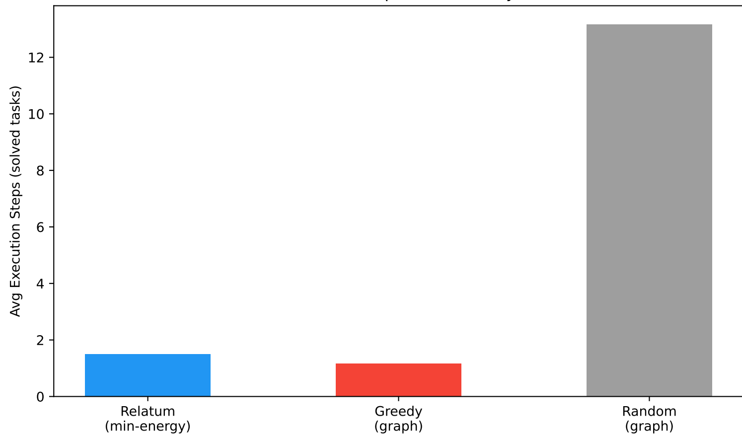
Execution Steps (Phase 2 only)
