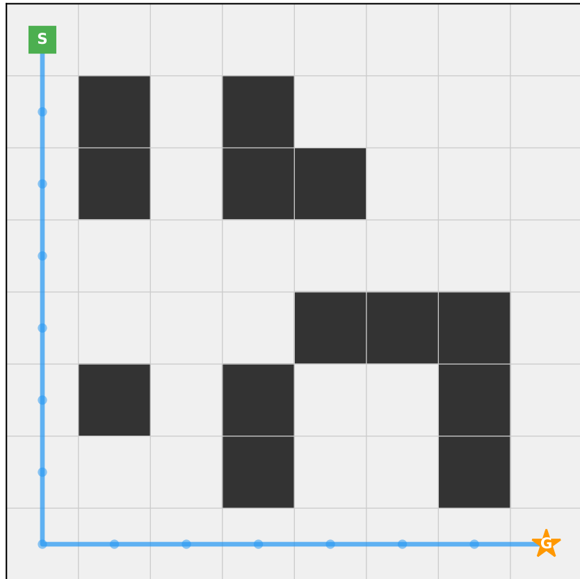
BFS (optimal) (14 steps)
