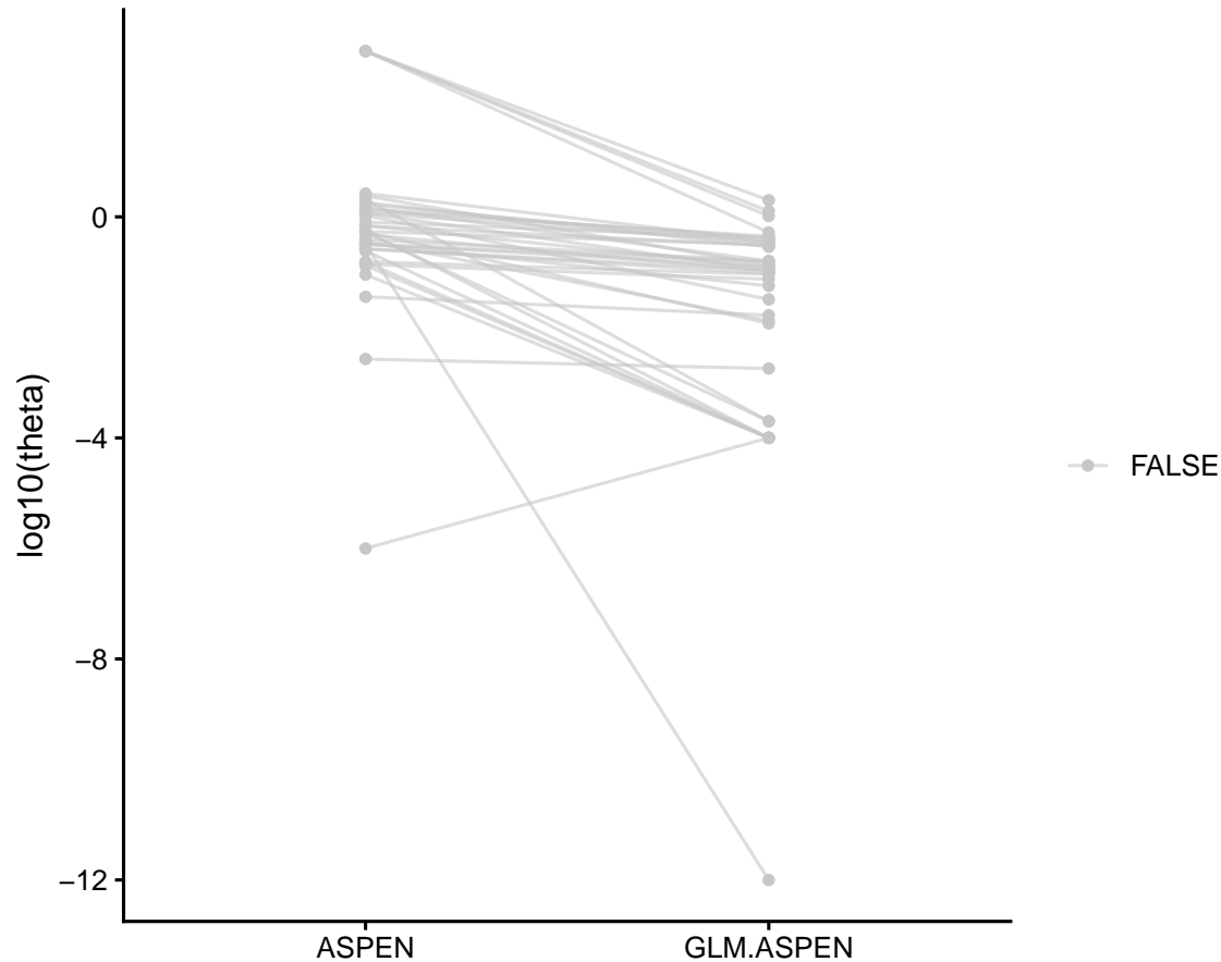
Smooth_Muscle F1_Aged – top |. log10(theta)| (n=40)
