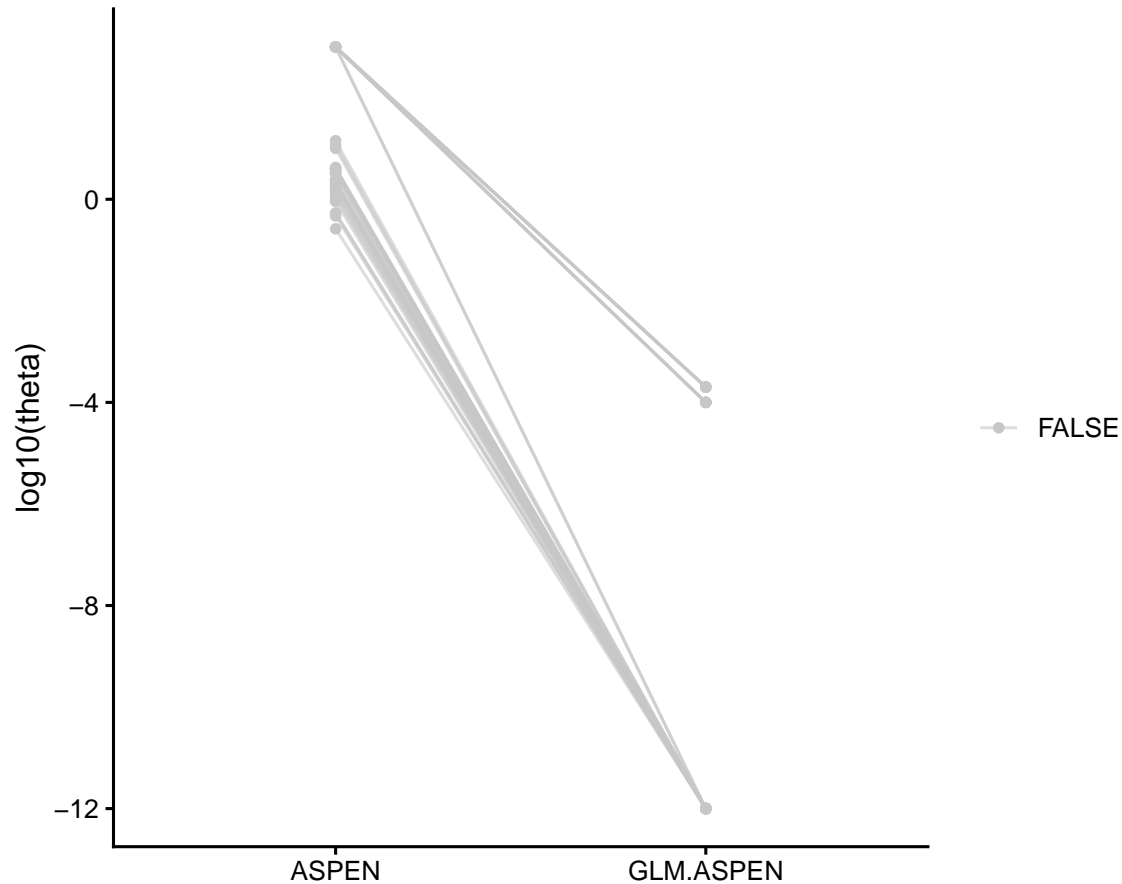
Mesothelial F1_Young – top |\log_{10}(\theta)| (n=40)
