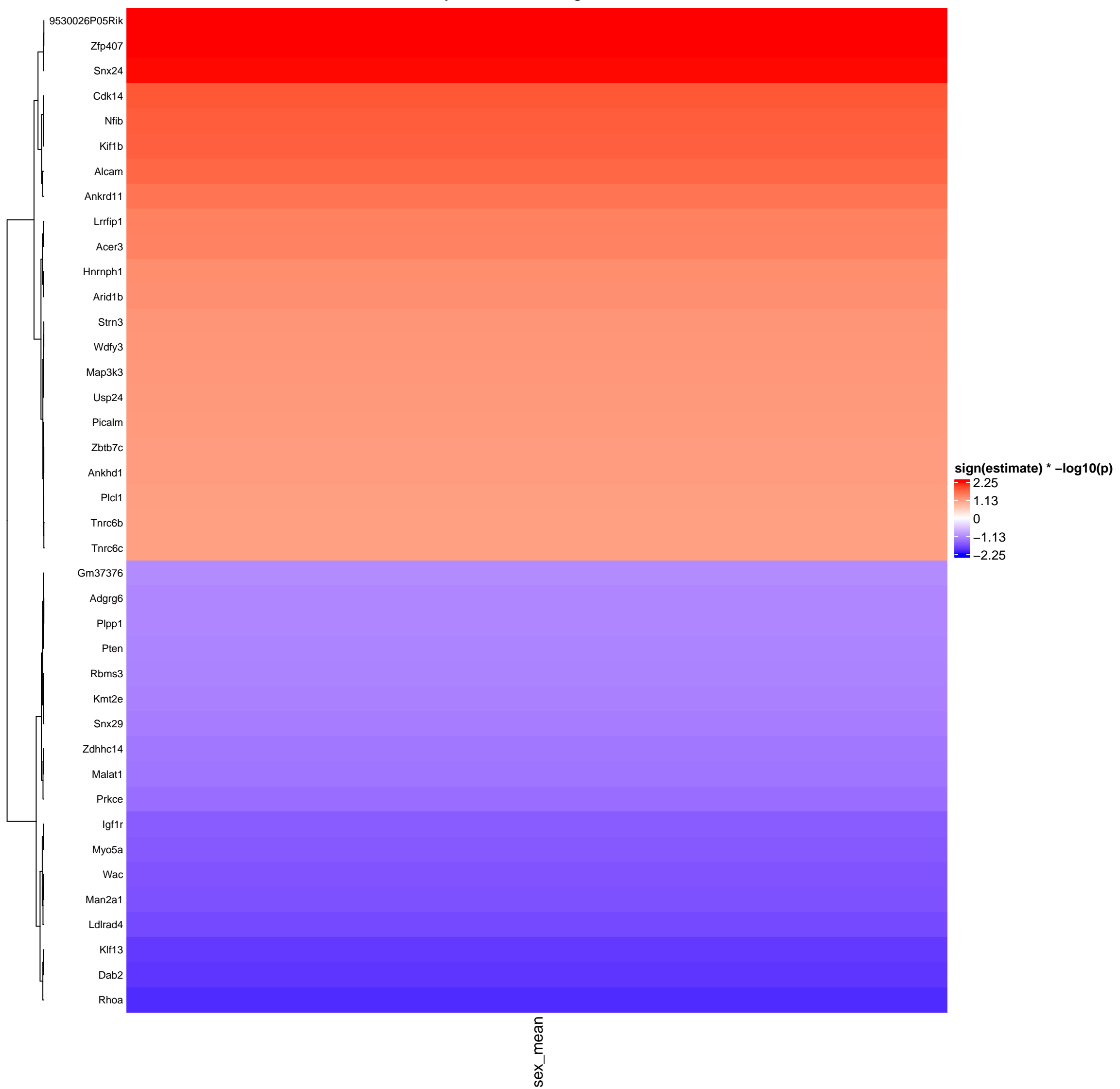
Myeloid__F1_Young – mean
