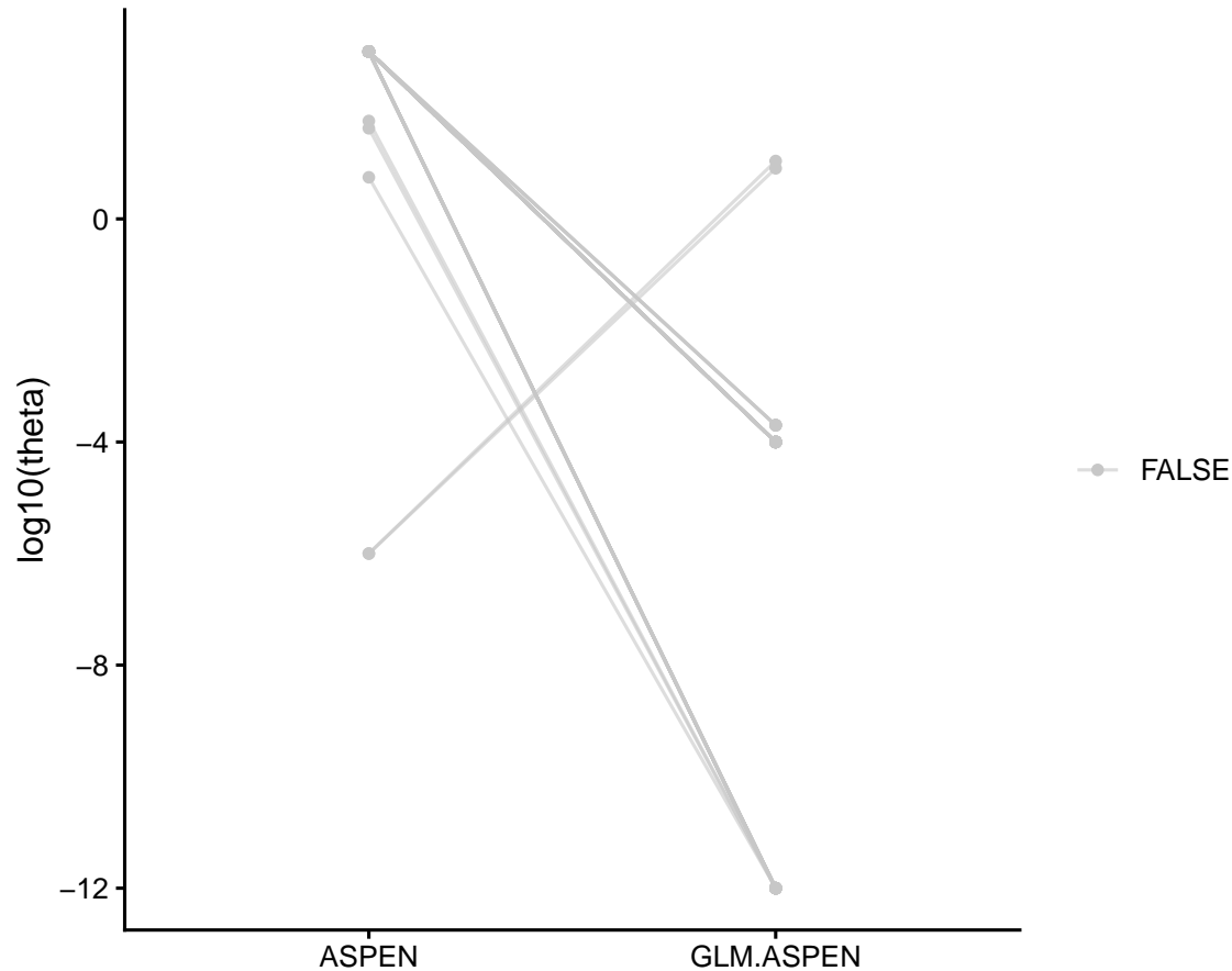
Pericytes F1_Aged – top |. log10(theta)| (n=40)
