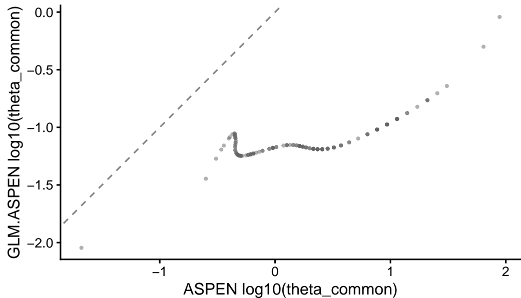
T_cell F1_Aged – trend target (theta_common)
