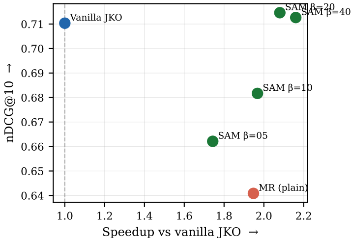
SAM-JKO: Quality-Speed Pareto (SciFact)
