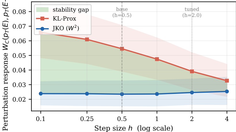
Stability gap shrinks as h \rightarrow \infty (verifies Corollary 3)
