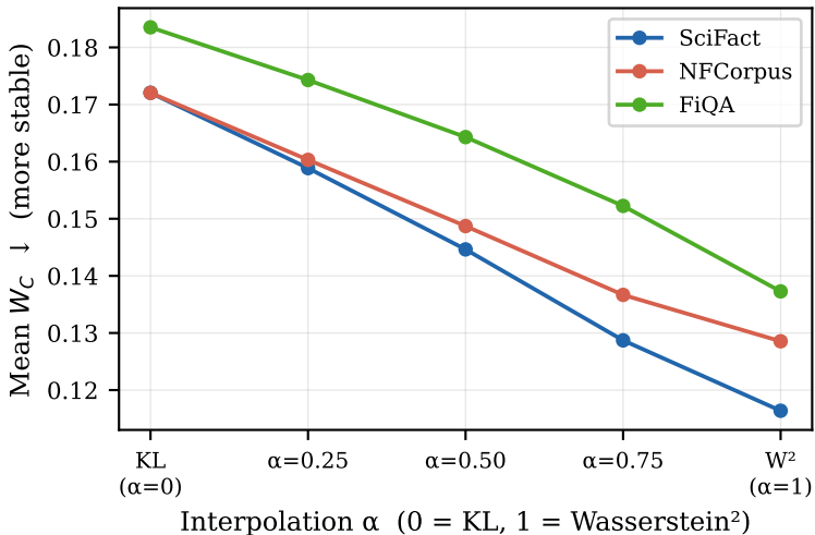
BW-JKO Stability vs. Interpolation Weight
