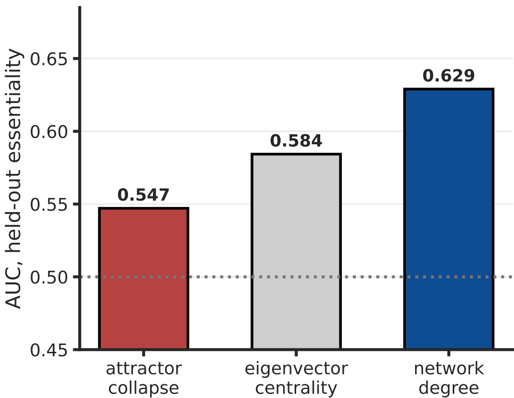
The proposed score loses to network degree
