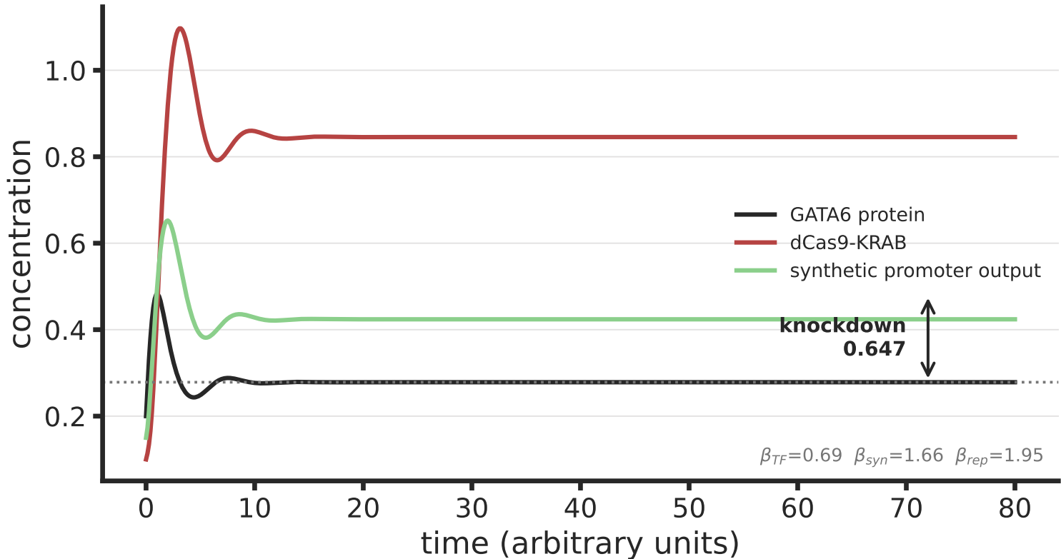
b Simulated kinetics of this circuit
