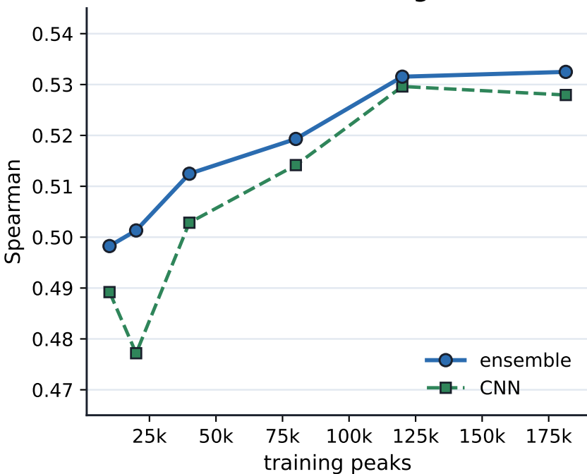
Promoter strength
