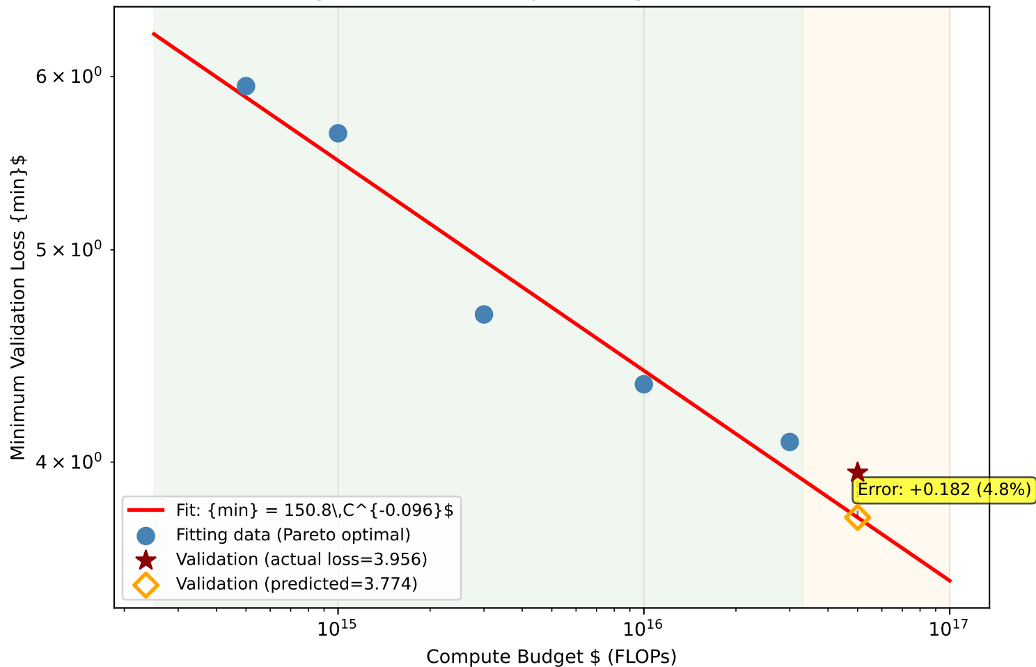
Scaling Law: Loss vs Compute Budget (with Validation)
