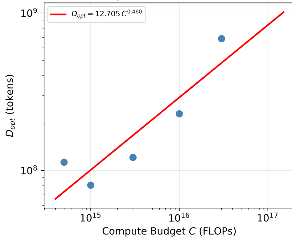
Optimal Dataset Size
