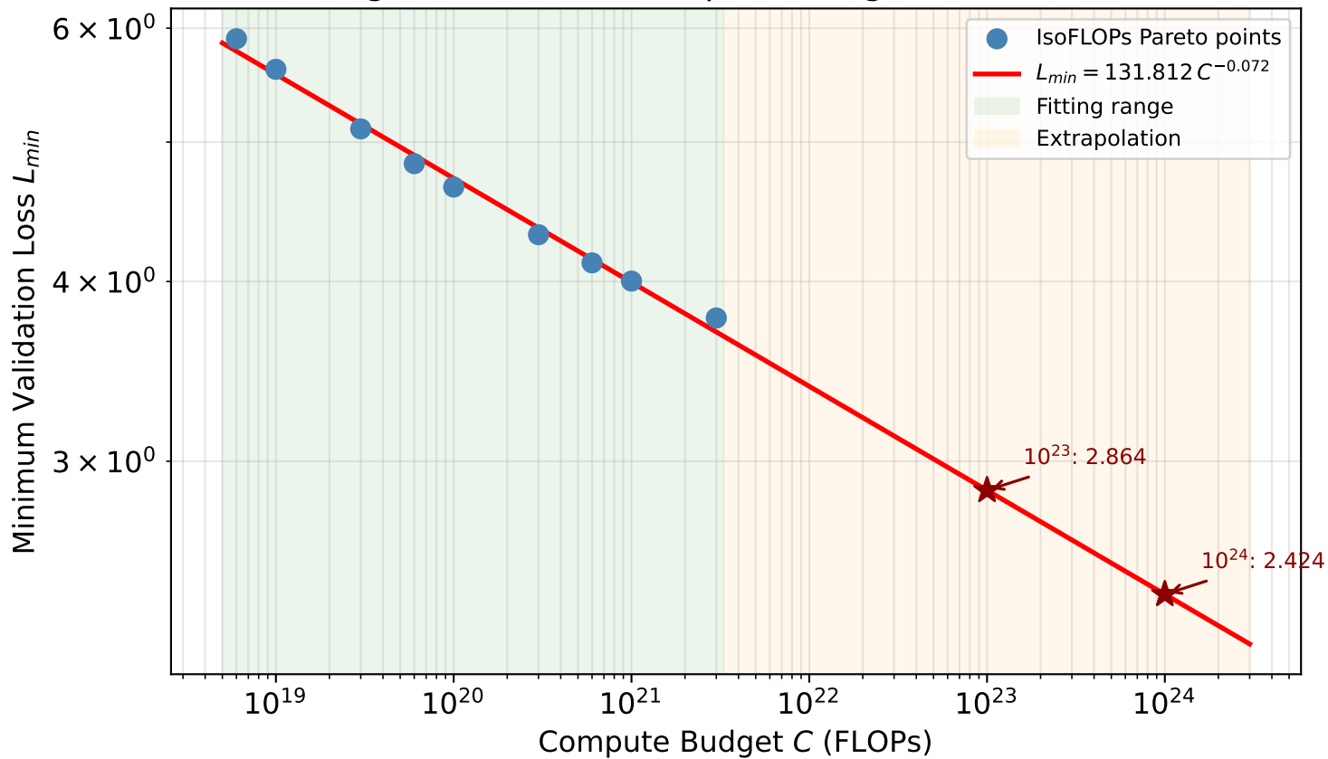
Scaling Law: Loss vs Compute Budget (Pareto Frontier)
