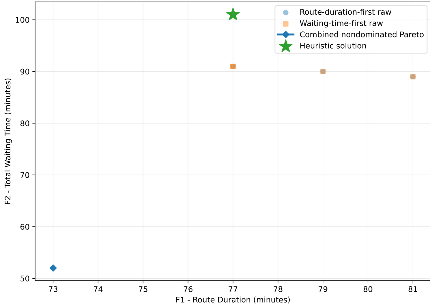
5-Part Instance - Case 1: Exact Pareto and Heuristic
