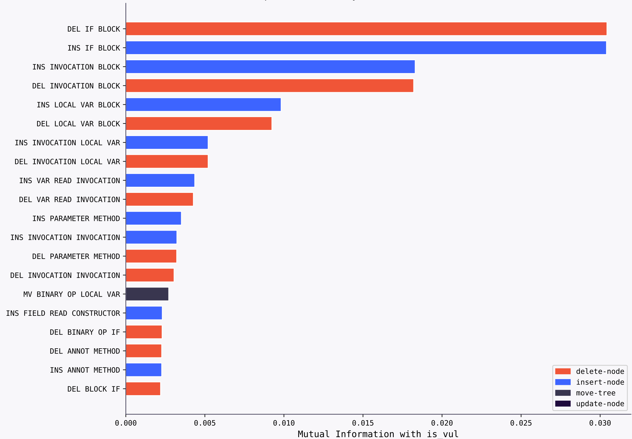
Top-20 Features by Mutual Information (BN1)
