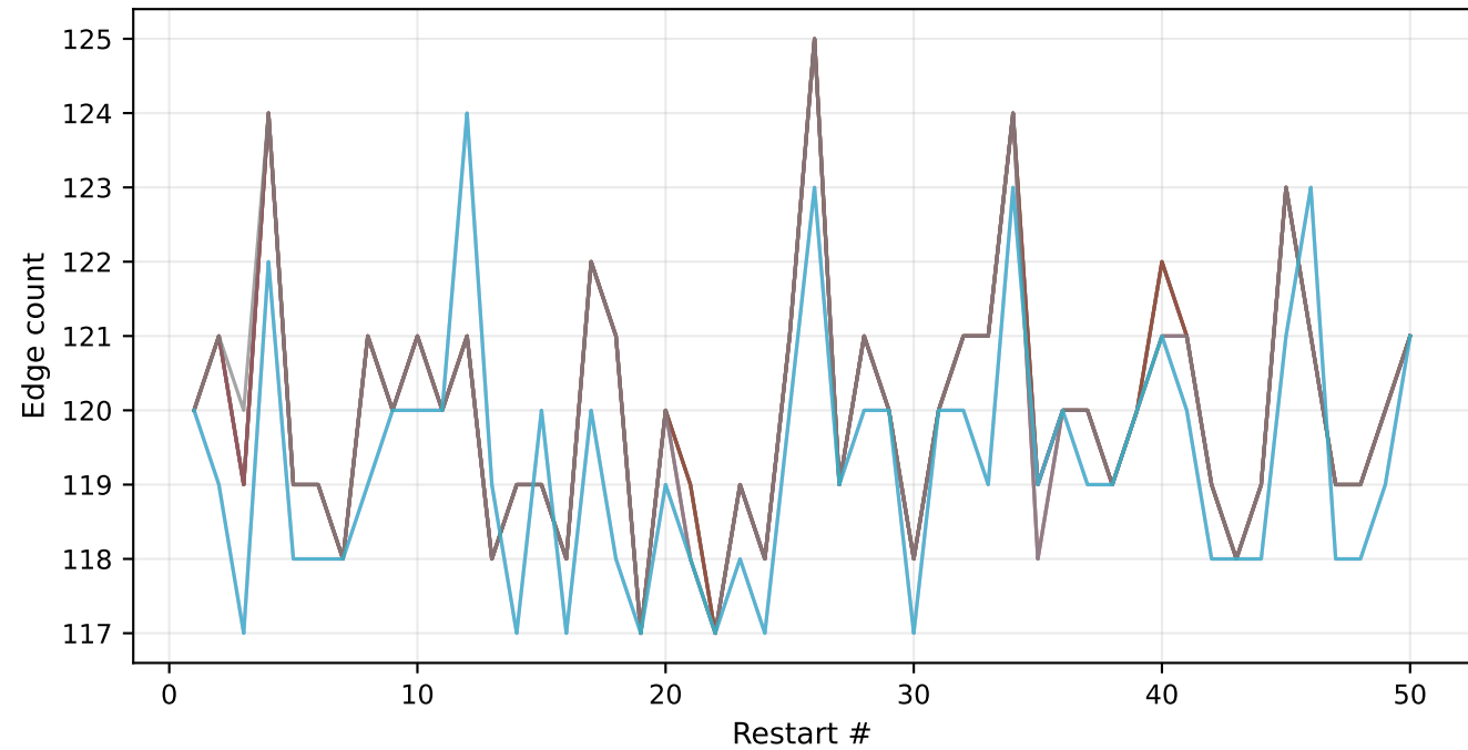
MI threshold = 100
