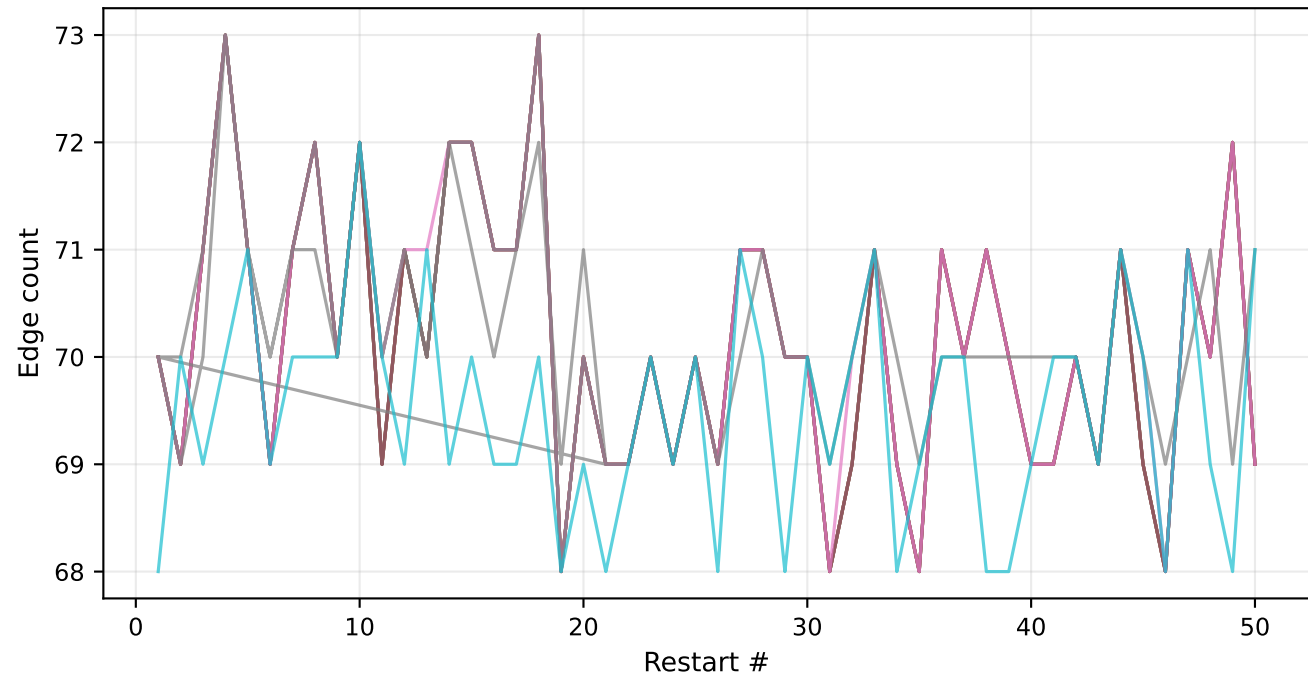
MI threshold = 50
