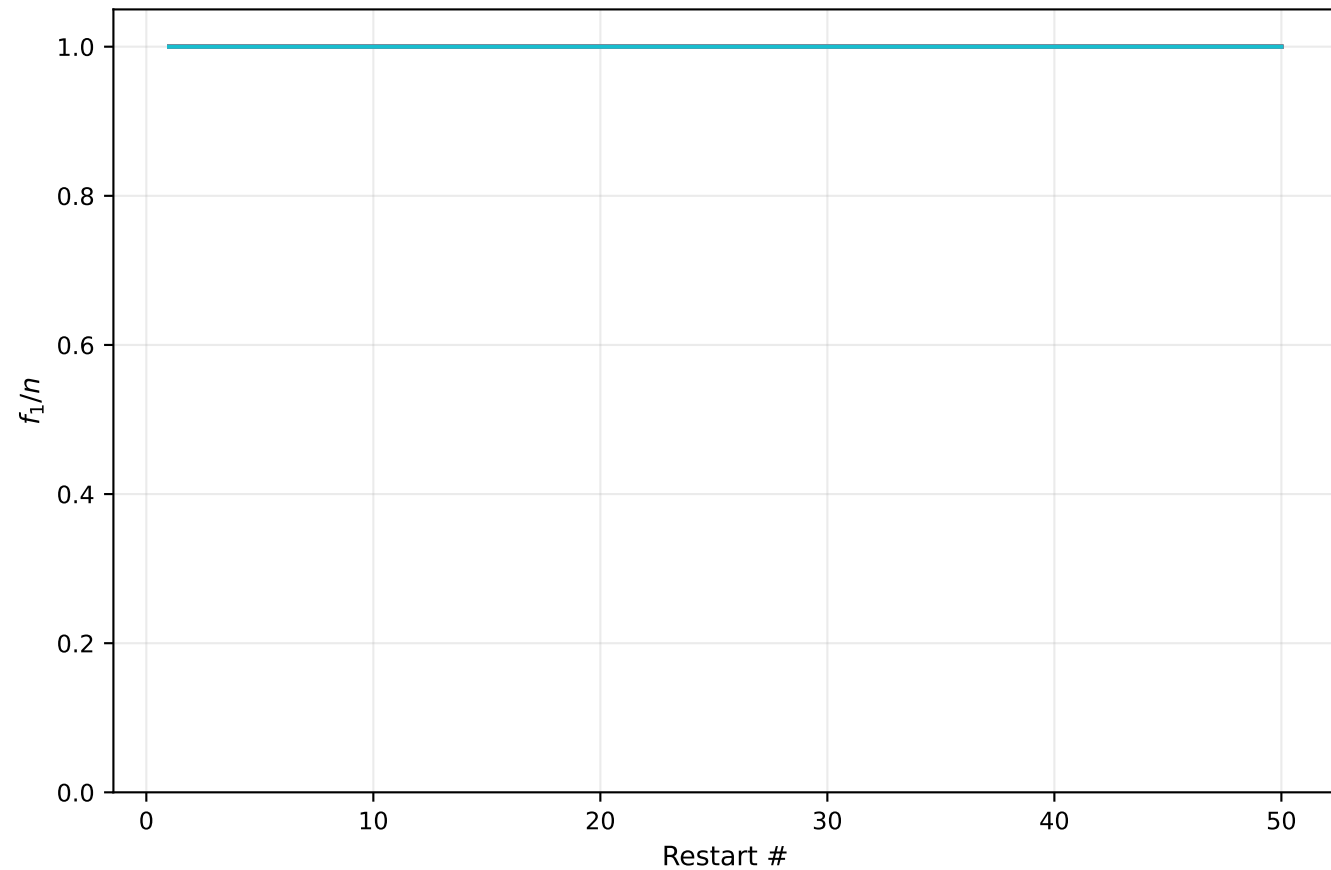
MI threshold = 100
