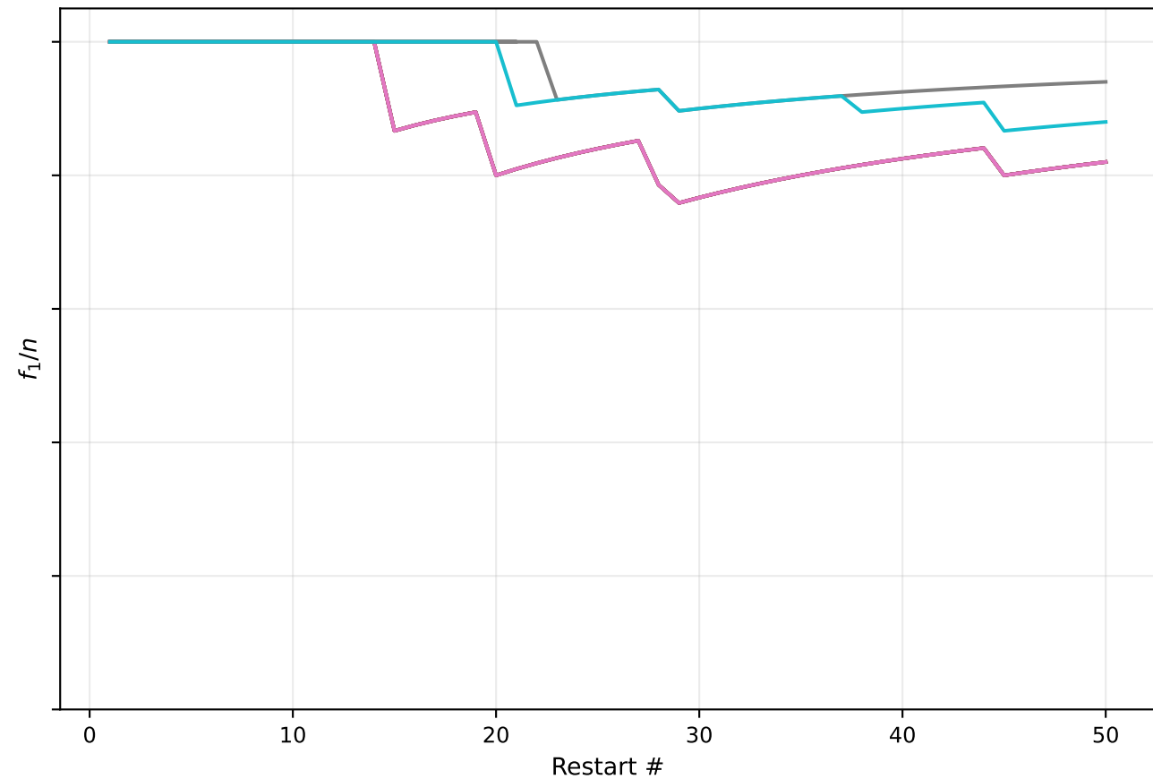
MI threshold = 50
