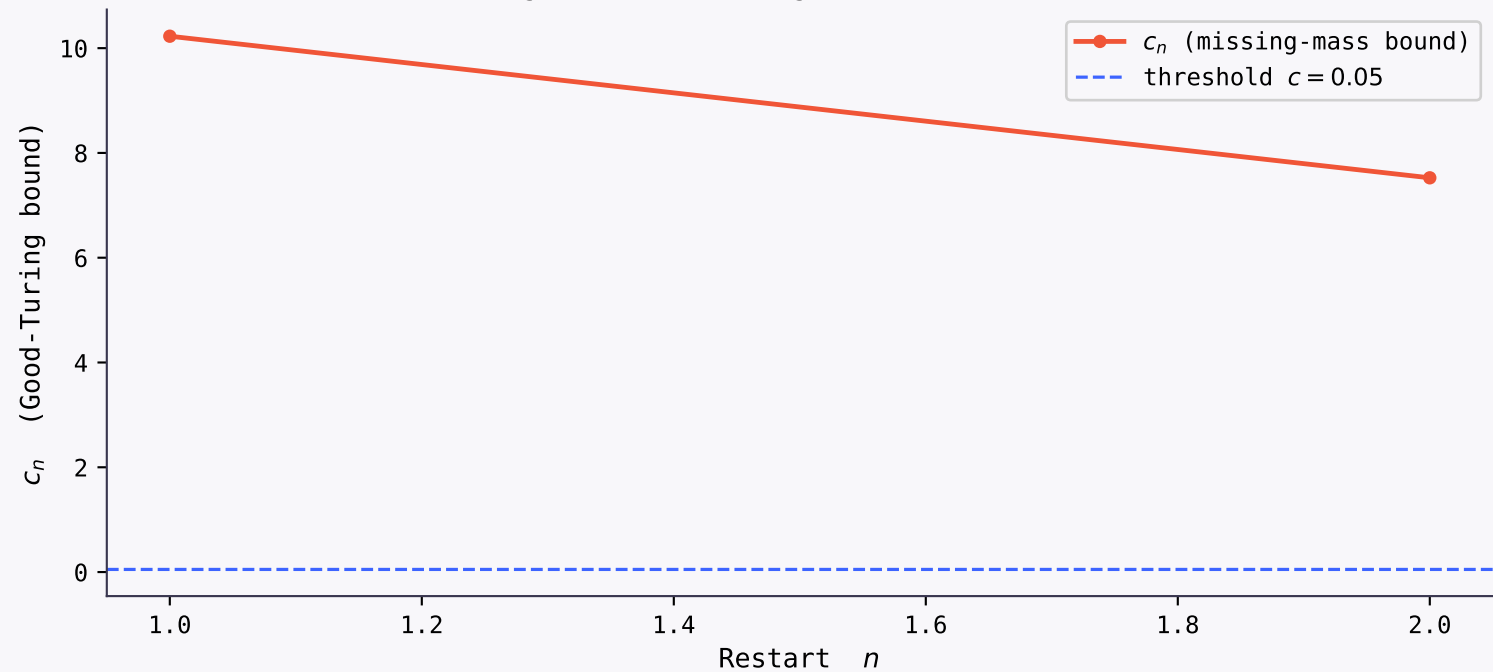
HCS Convergence – Missing-Mass Bound vs. Restarts
