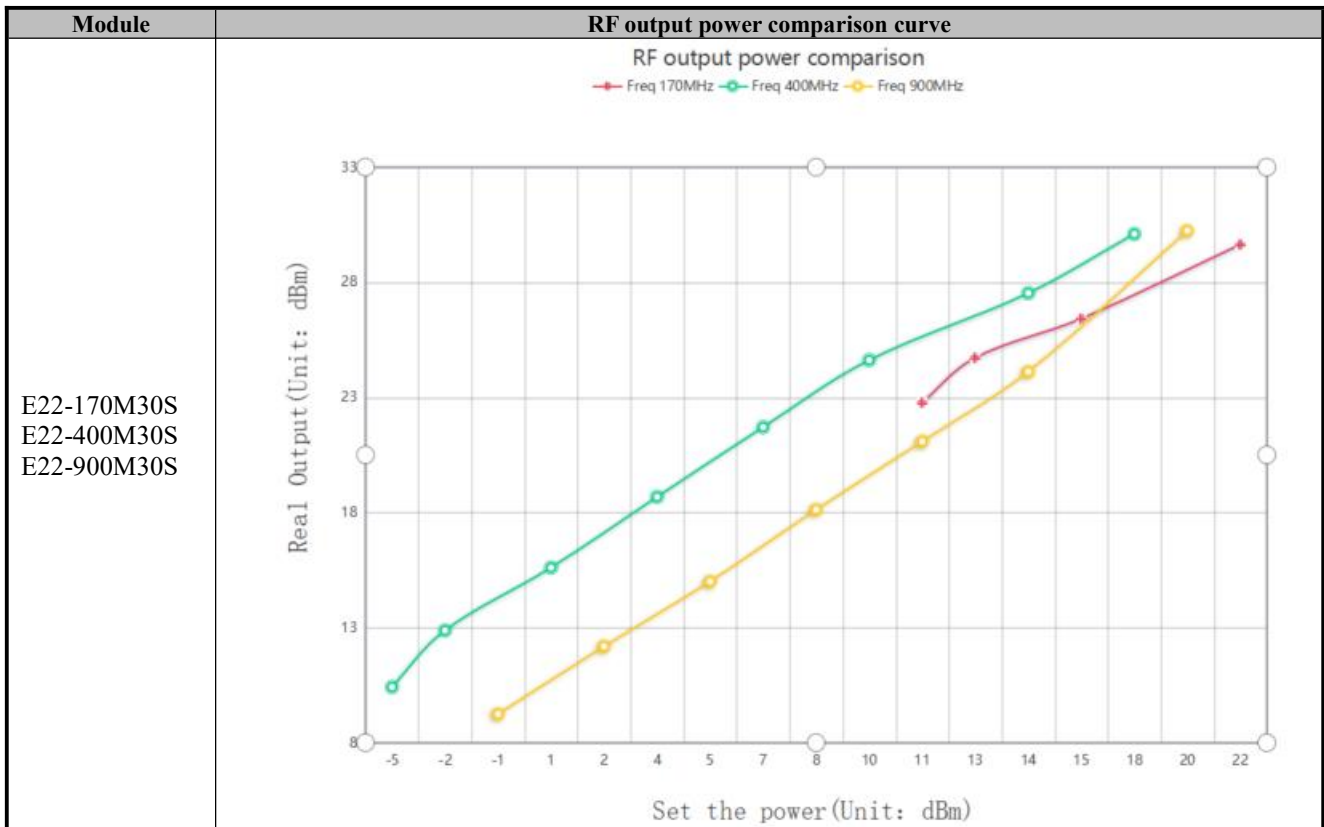
Chart 2 [The RF output power control table]
