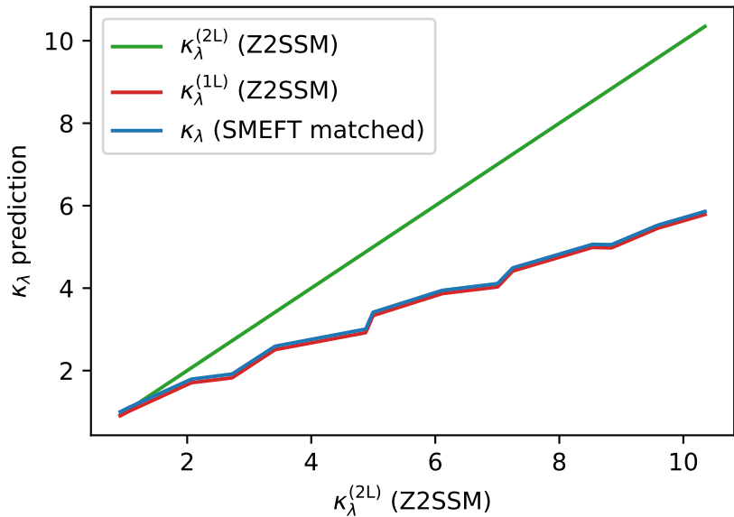
\kappa_\lambda comparison
