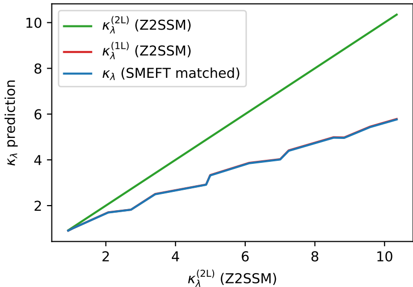
\kappa_\lambda comparison
