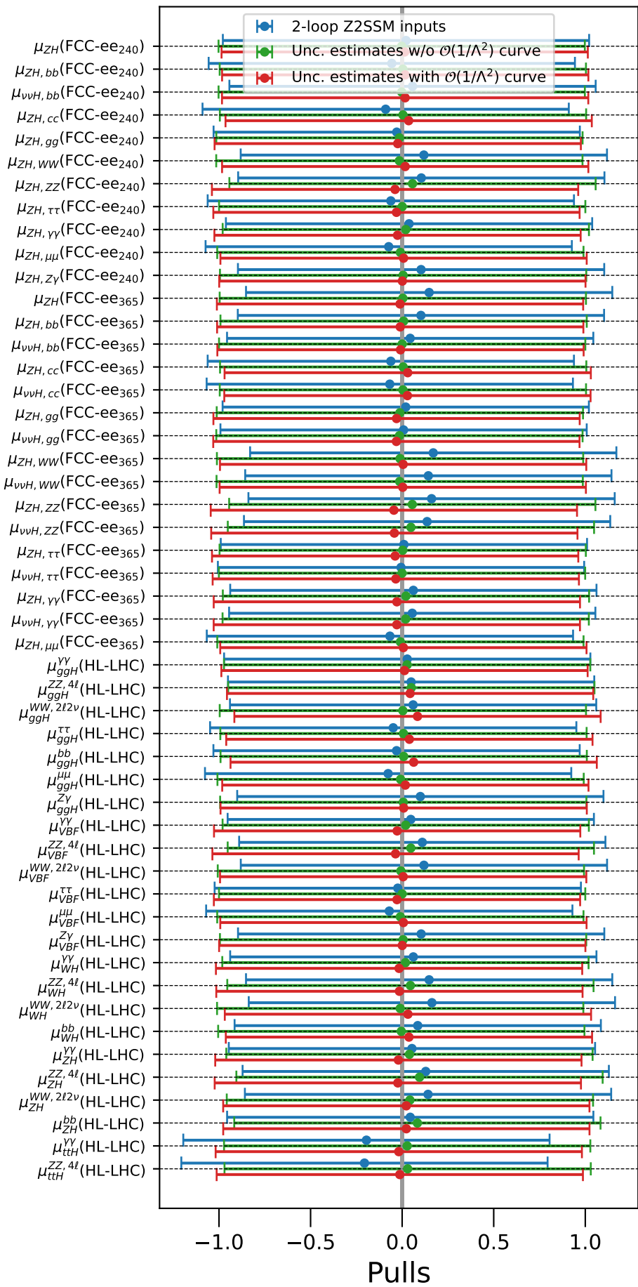
Z2SSM (BP 0), FCC-ee 240 + FCC-ee 365
