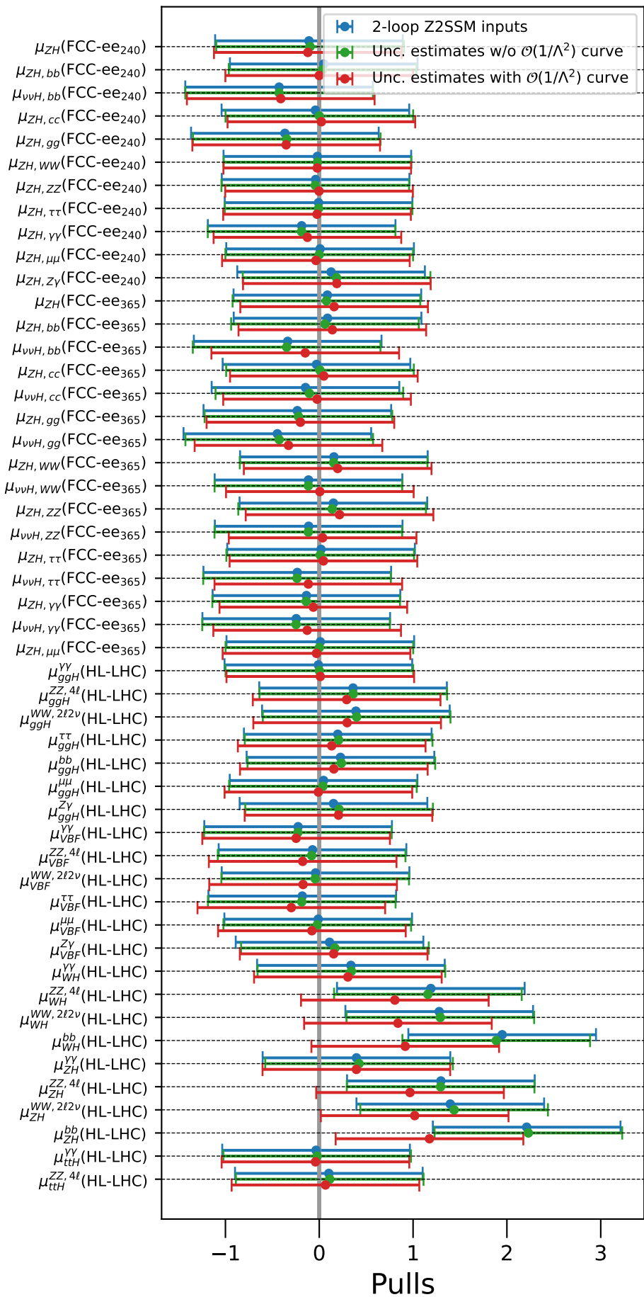
Z2SSM (BP 3), FCC-ee 240 + FCC-ee 365
