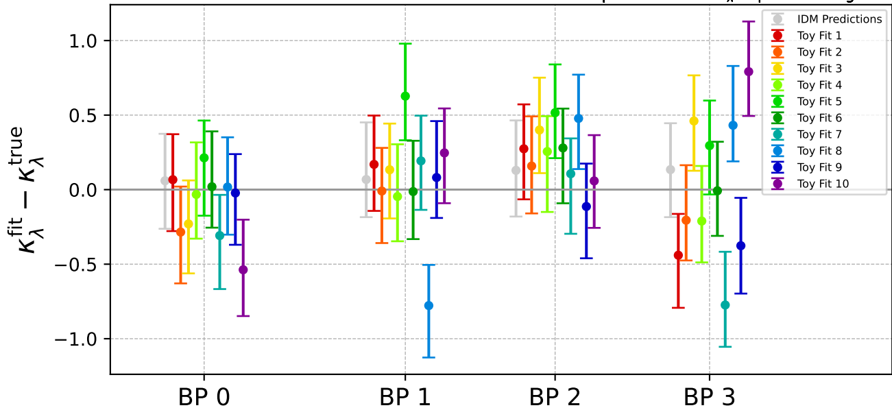
IDM inputs: 1L BSM + \kappa_\lambda -dependent diagrams
