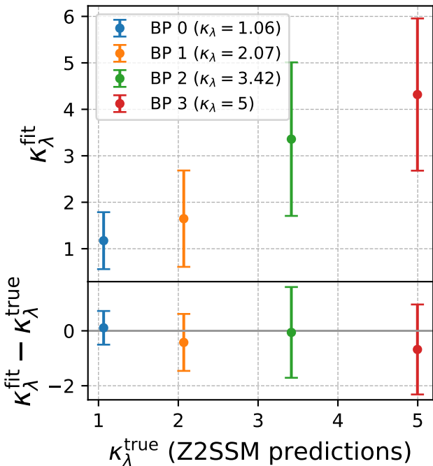
Estimates with \mathcal{O}(1/\Lambda^2) curve
