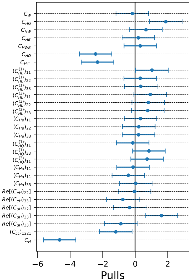
IDM (BP 1), FCC-ee 240 + FCC-ee 365 + \kappa_\lambda at HL-LHC
