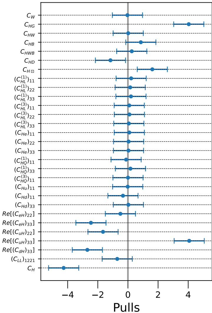
IDM (BP 3), FCC-ee 240
