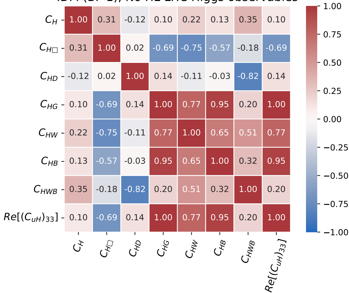
IDM (BP 1), No HL-LHC Higgs observables
