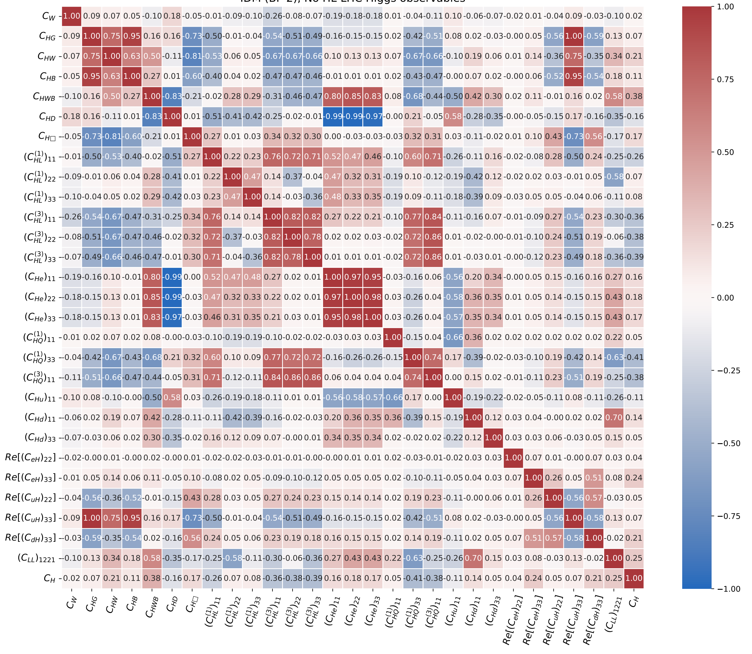
IDM (BP 2), No HL-LHC Higgs observables
