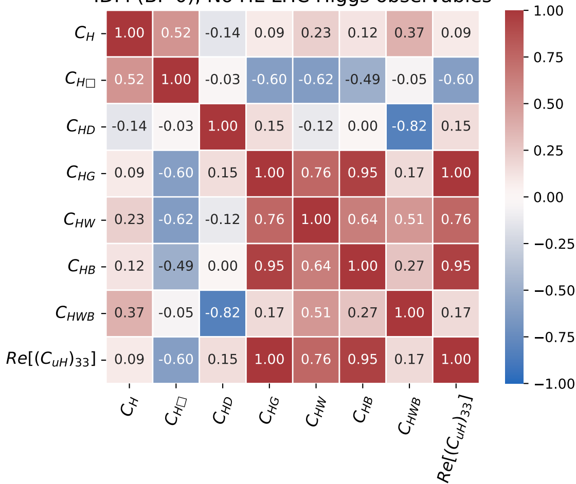
IDM (BP 0), No HL-LHC Higgs observables
