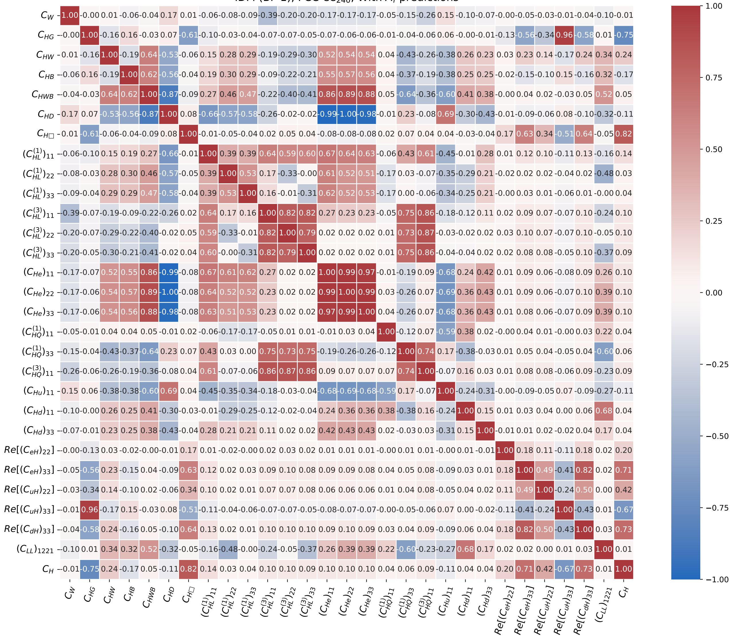
IDM (BP 1), FCC-ee 240 , With A_f predictions
